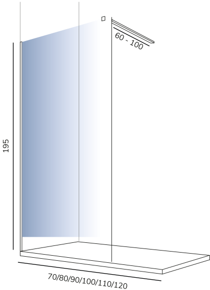
Acabado Aluminio y Negro Mate. Aluminum and Black Matt finishes.
